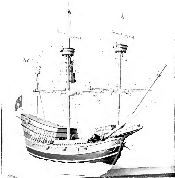
FRENCH SHIP OF WAR. C. 1550.
